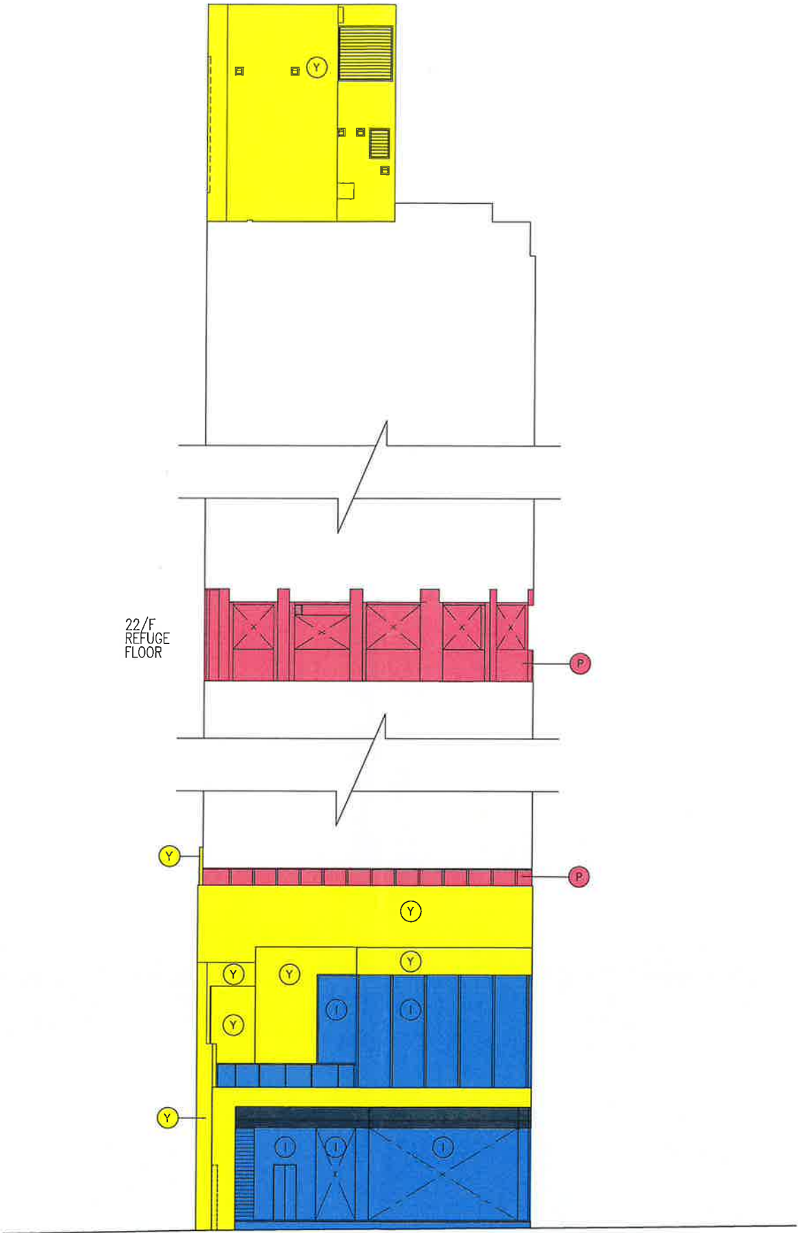
ELEVATION FROM LI TAK STREET (FOR IDENTIFICATION PURPOSE ONLY) (SCALE 1:200)
