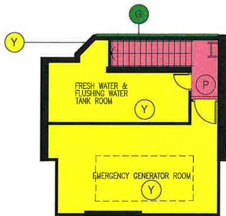
FLOOR PLAN AT +105.120 (FOR IDENTIFICATION PURPOSE ONLY) (SCALE 1:150)
